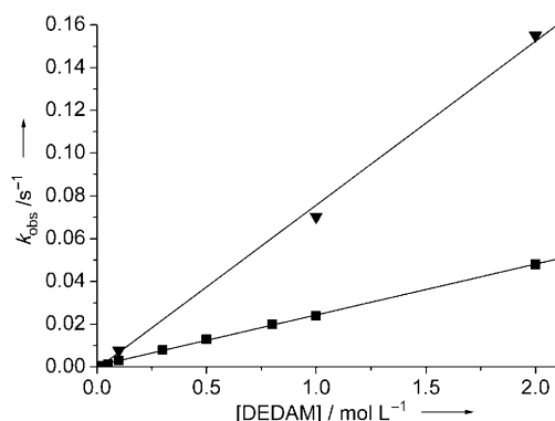
Figure 1. k_{\text{obs}} versus [DEDAM] ( c = 0.005\text{ M} – 2\text{ M} ) for the RCM reaction with 1 (squares, R^2 = 0.999 for seven pairs of data) or 2 (triangles, R^2 = 0.998 for five pairs of data). T = 40^\circ\text{C} .
